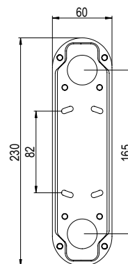
WALL PLATE
