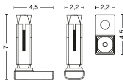
FIXATION BRACKET FOR BENCHES WIDTH 4,5 CM DEPTH 2,2 CM HEIGHT 7 CM
