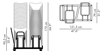
LARGE TRANSPORT DOLLY: (FOR 40 CHAIRS)
